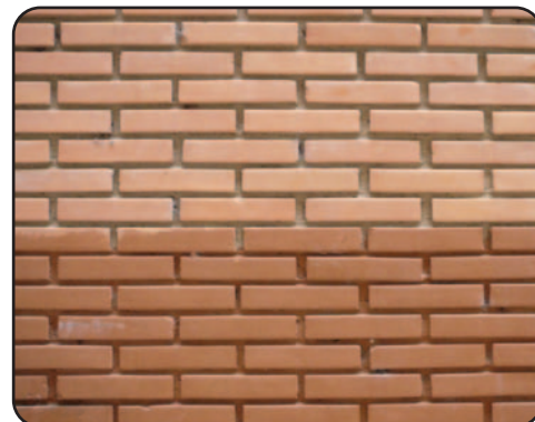
Zahabiya REPECOAT coated on the upper half. The surface looks dry even after rain.
